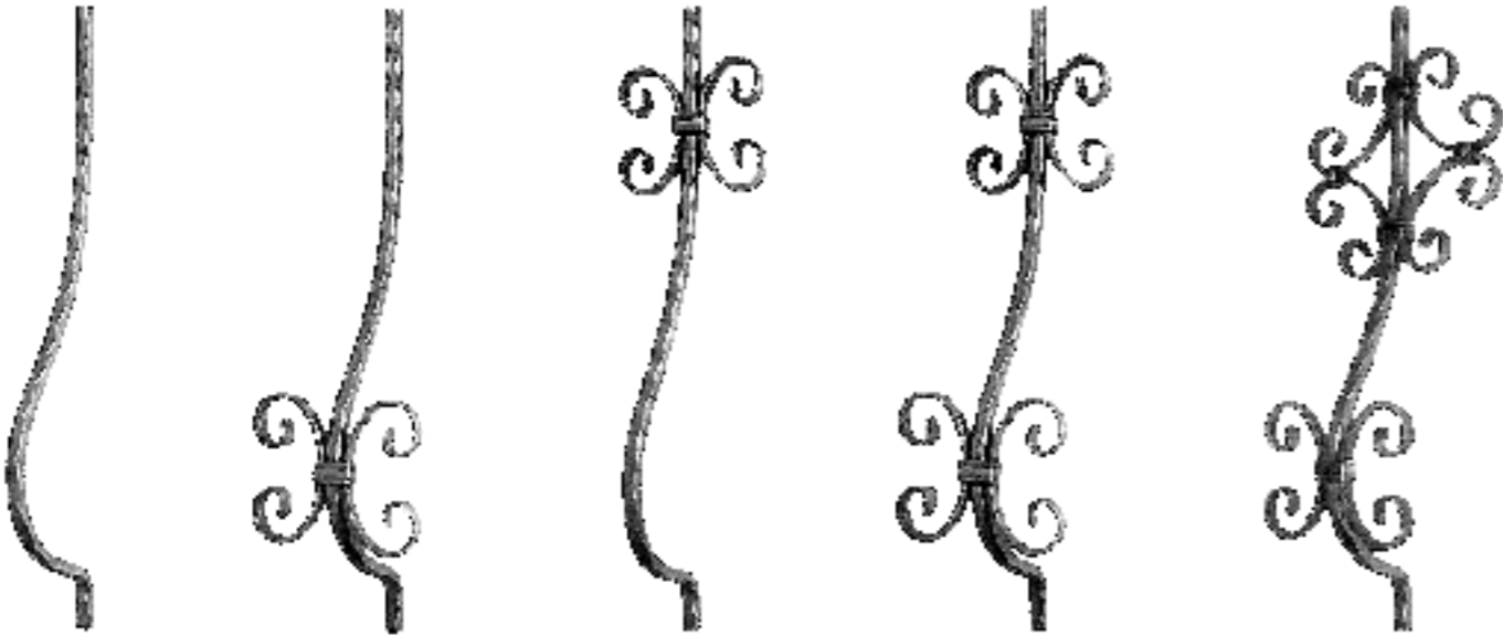
C-690 1,2x50x10 0,62kg. C-691 13x50x10 0,93kg. C-692 13x50x10 0,93kg. C-693 13x50x10 1,24kg. C-694 18,5x50x10 1,54kg.
