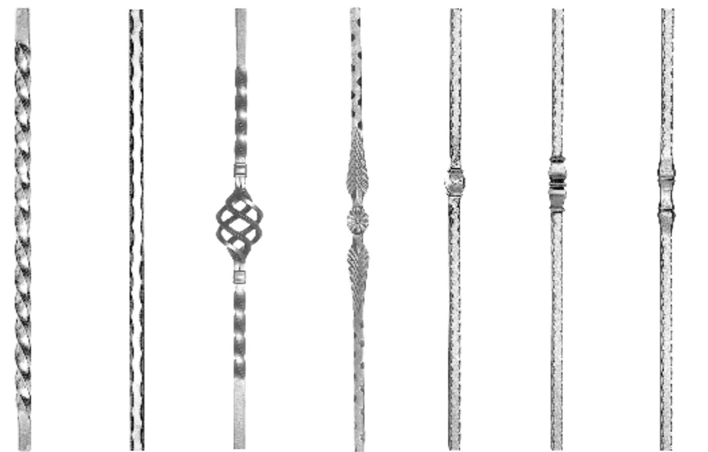
N-100x24 2,4x100 4,52kg. İ-100x24 2,5x100 4,52kg. K 100-1x24 2,4x100 4,53kg. B-605 5x41 4,24kg. B-101 4x6 4,63kg. B-103 4x13 5,04kg. B-105 3,5x13 4,71kg.
